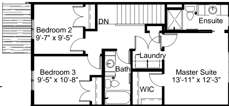
Second Floor Plan 709 SQFT 8'-1" Second Floor Ceiling
