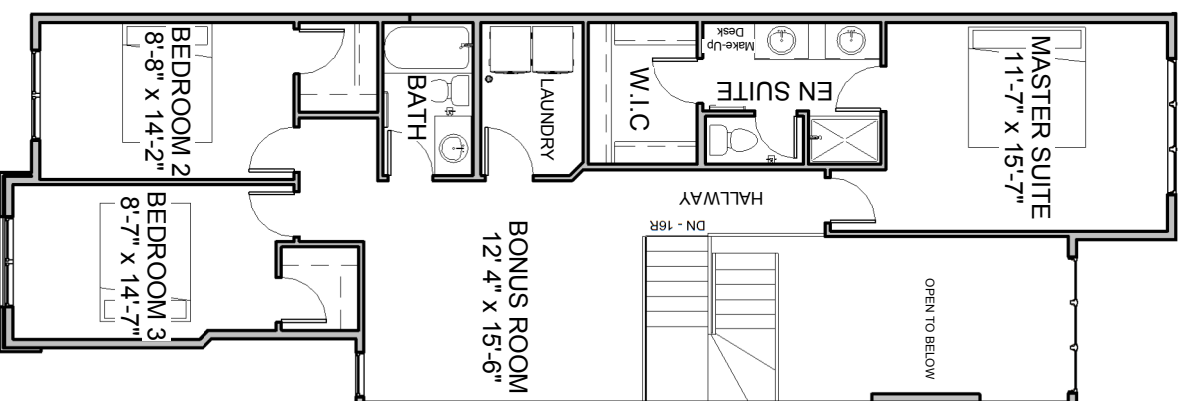
SECOND FLOOR 1060 SQFT 8'-1" CEILING HEIGHT
